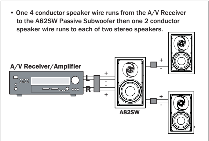
Figure 3.6 - Wiring: Amplifier to Speaker-Passive Subwoofer
